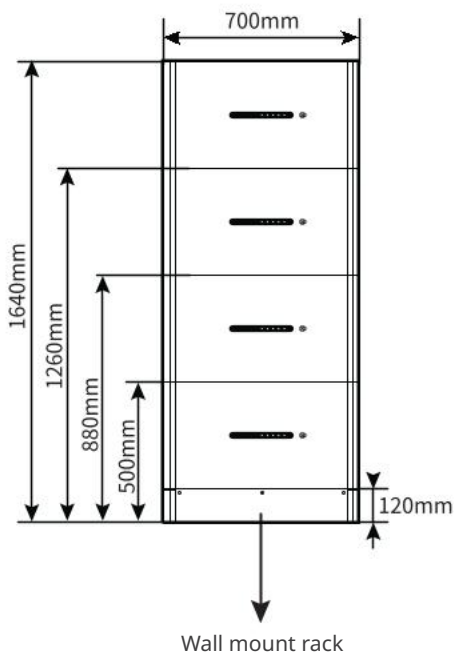
Battery group dimensions (wall-mount installation)
