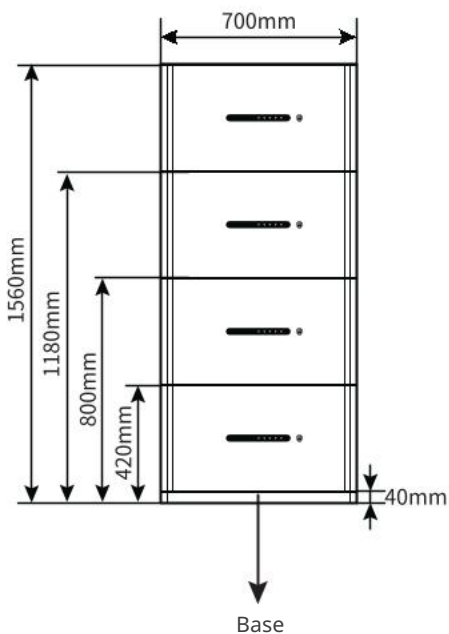
Battery group dimensions (ground installation)
