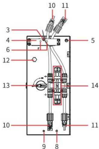
Right View
